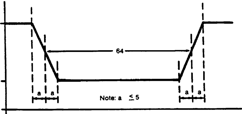
Figure 1.-DPSK Phase Characteristic
